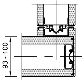
1. 90° CORNER PANEL (EE)
