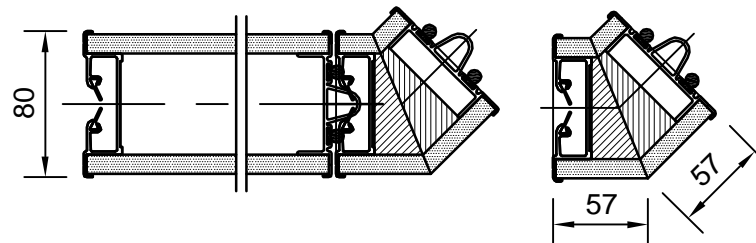
1. 45° CORNER PANEL (EE)
