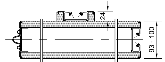
3. JUNCTION PANEL (EE)
