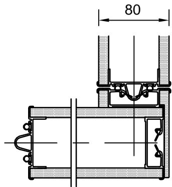
1. 90° CORNER PANEL (EE)
