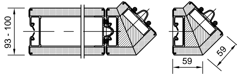
1. 45° CORNER PANEL (EE)
